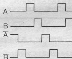
(a) 1相励磁
