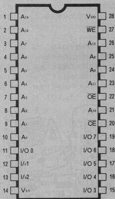
図4 HM62256LP-12
